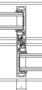
Sill Detail
