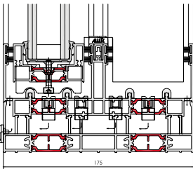
Sill Detail
